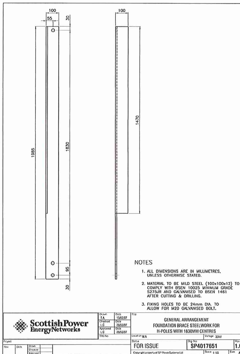
Figure 31 General Arrangement Foundation Brace Steelwork "H" Pole 1830mm Centres (Drawing 4017651)
